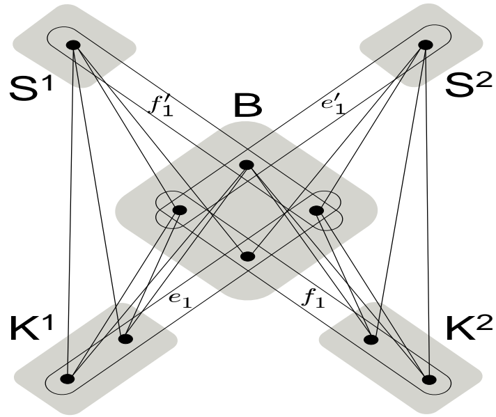
Figure 5: The hypergraph H_1 defined in Example 7.12. (Edges totally contained in other edges are not shown.)
