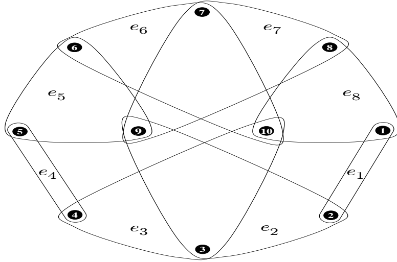
Figure 1: The hypergraph H_{AG} , which is the structure of the CSP instance P_{AG} , defined in Example 2.2.
