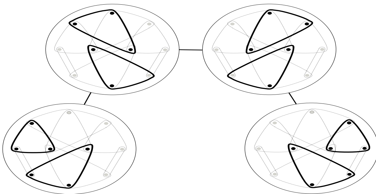
Figure 4: The spread cut defined in Example 7.9 for the hypergraph H_{AG} defined in Example 2.5
