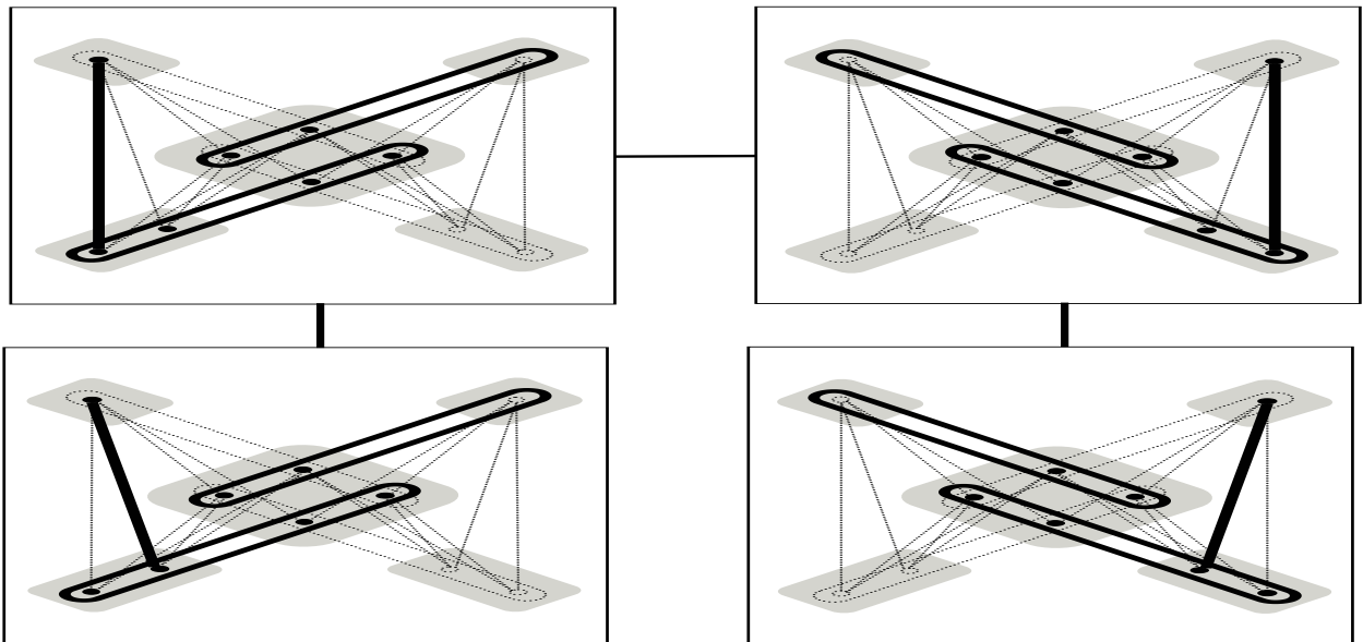
Figure 6: The spread-cut decomposition \Xi_1 defined in Example 7.12 for the hypergraph H_1
